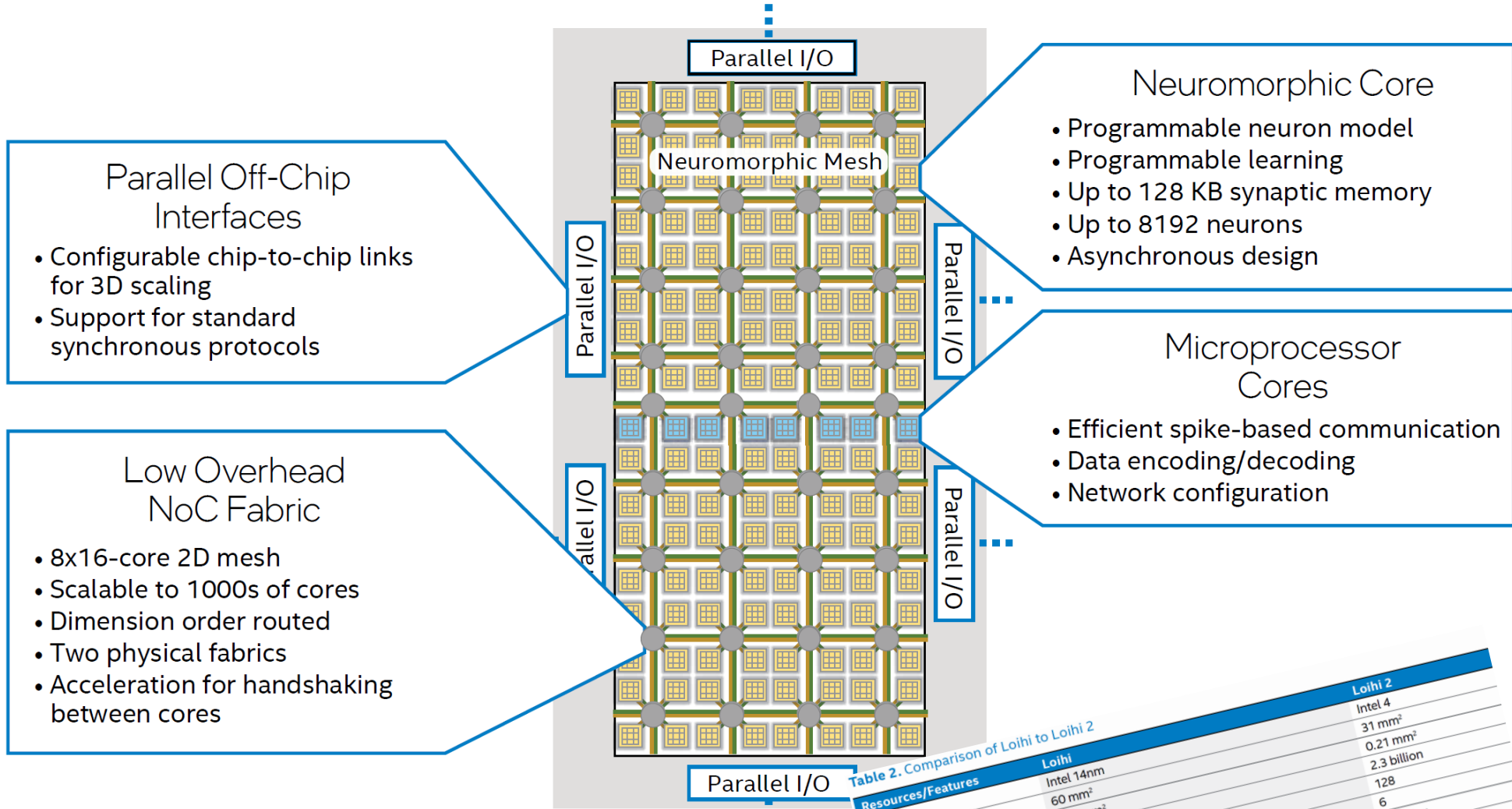
Figure 1. Loihi 2 chip architecture.
